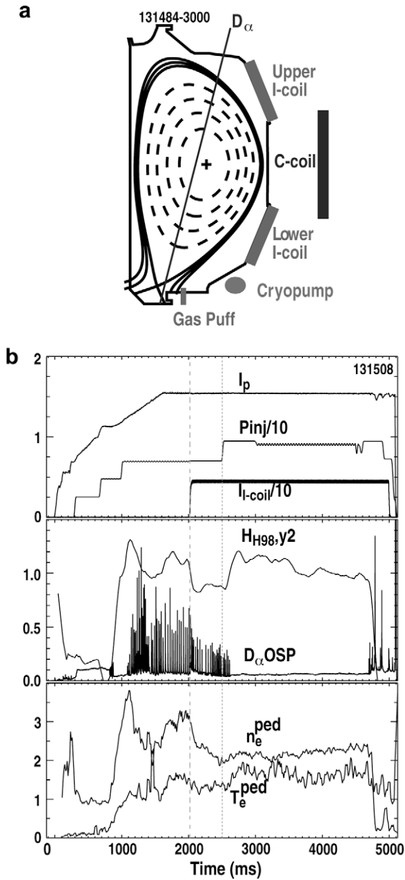
Fig. 1. Overview of operational parameters for discharges in this study including: (a) plasma and coil geometry of the high triangularity ISS showing the optimal position of the outer strike point for pumping, the location of the D_\alpha line integrated measurement, and the locations of the I- and C-coils, and (b) temporal evolution of basic discharge parameters including plasma current [ I_p (MA)], injected neutral beam power [ P_{inj} (10 MW)], I-coil current [ I_{coil} (10 kAt)]; confinement enhancement factor H(98,y2) and divertor outer strike point D_\alpha intensity ( 1 \times 10^{20} phot/m 2 /s/str); pedestal electron density [ n_e^{ped} ( 10^{19} m -3 )] and temperature [ T_e^{ped} (keV)]. I-coil on and power increase times marked by vertical dashed and dotted lines, respectively.
