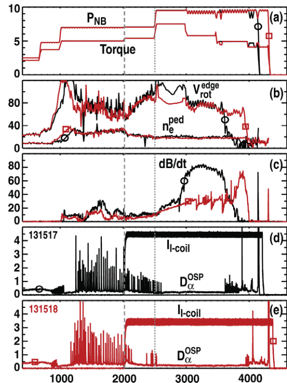
Fig. 2. Comparison of parameters from plasmas using one vs. two I-coil rows in which input NBI torque is reduced in steps during the RMP phase for upper I-coil alone at 4.5 kAt and low density (black-circle), and both I-coils at 3.5 kAt and low pedestal density (red-square), including: (a) injected co-current neutral beam torque (N-m) and injected NB power (MW), (b) pedestal density ( 10^{18} m -3 ) and toroidal rotation in the edge pedestal (km/s), (c) amplitude of core MHD activity (T/s) and (d-e) outer divertor D_\alpha intensity ( 2.5 \times 10^{19} phot/m 2 /s/str) and I-coil current (kAt). I-coil on and power increase times marked by vertical dashed and dotted lines respectively. (For interpretation of the references to colour in this figure legend, the reader is referred to the web version of this article.)
