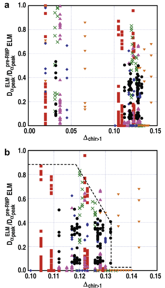
Fig. 4. Peak magnitude of ELM transient on outer strikepoint D_\alpha signal as a function of the width in normalized flux of the vacuum island overlap region with Chirikov parameter > 1.0 [ \Delta\Psi_{N(\text{chir}>1)} ] for multiple transients in the discharges from Fig. 3(a–f). (a) The value of ELM size plotted is normalized to the maximum size of the ELMs in the H-mode phase prior to application of the I-coil RMP field for each discharge, and (b) plot expanded for timeslices with the RMP coil on. Transients from a given discharge in Fig. 3 are marked with the same color and symbol used to identify the discharge in Fig. 3.
